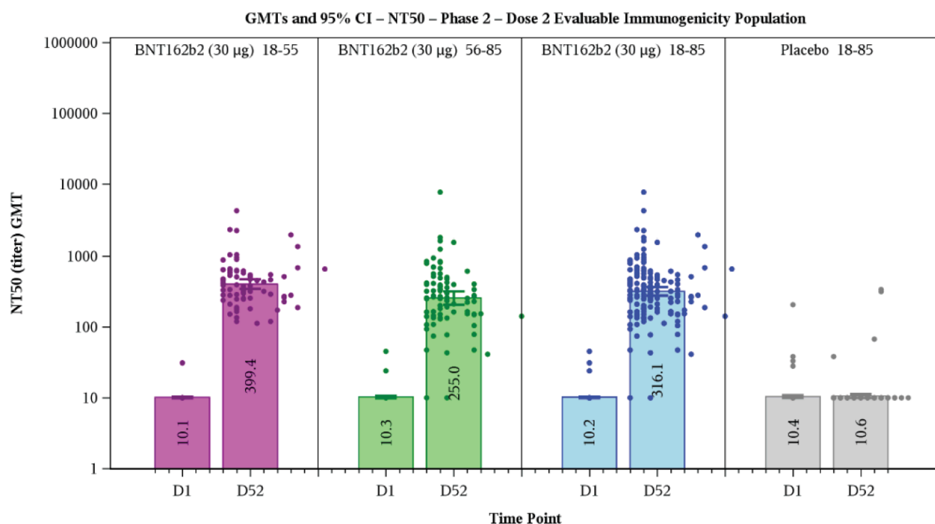
Figure 16. Geometric Mean Titrers and 95% CI: SARS-CoV-2 Neutralization Assay – NT50 – Phase 2 – Dose 2 Evaluable Immunogenicity Population
