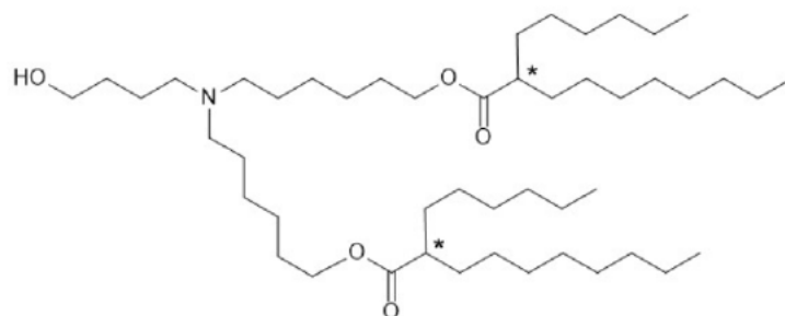
Figure 4 ALC-0315 structure
