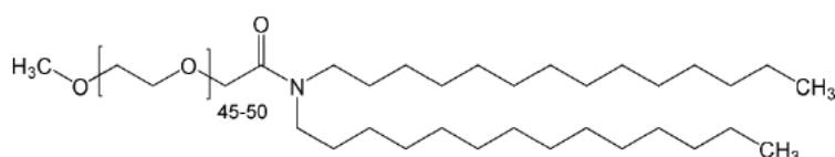
Figure 6 ALC-0159 structure
