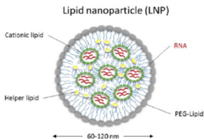
Figure 1 Lipid nanoparticle (LNP)
