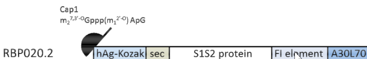
Figure 1 General structure of BNT162b2 RNA
